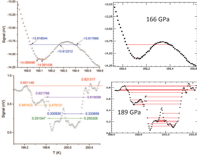
FIG. 4: Right panels: the portion of the right panels of the curves of Fig. 3 within the rectangles, to higher resolution. The red lines show anomalous coincidences discussed in ref. [1]. The left panels show the corresponding portions of the curves claimed to be true by the authors in ref. [3]. Note that the shapes of the curves on the left and right panels are identical, the claimed disagreement is in the third significant figure.
